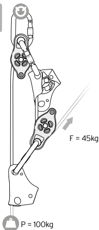
4f. 3:1 hauling system with progress capture
