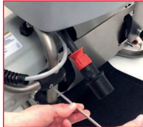
2. Unscrew the second screw in the accelerator control with an Allen wrench no. 4. Please watch out not to lose the self-locking nut.
