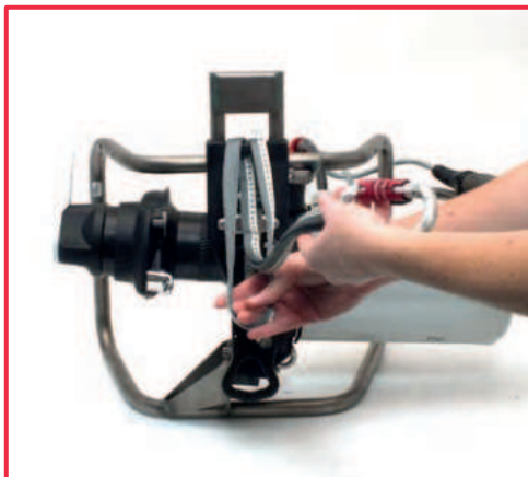
3. Remove the stop from upper anchorage point.
